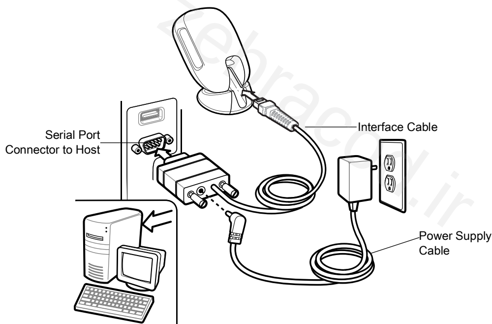
Figure 20 RS-232 Connection
