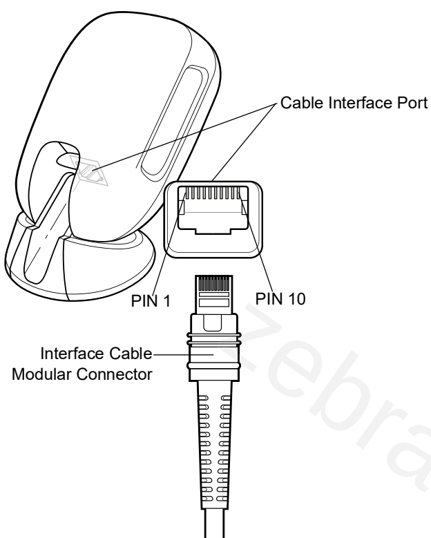
Figure 18 Scanner Cable Pinouts
