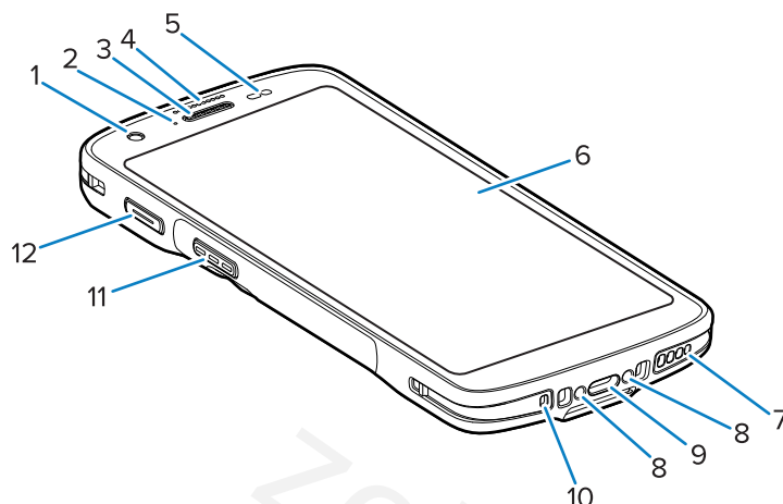
Figure 1 Front View
