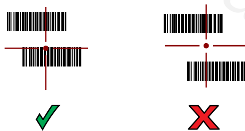
Figure 16 RS6000 Pick List Mode with Multiple Barcodes in Aiming Pattern
