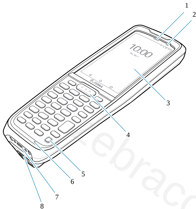
Figure 1 Front View
