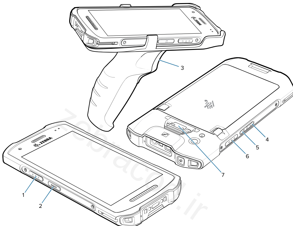
Figure 11 Remappable Keys
