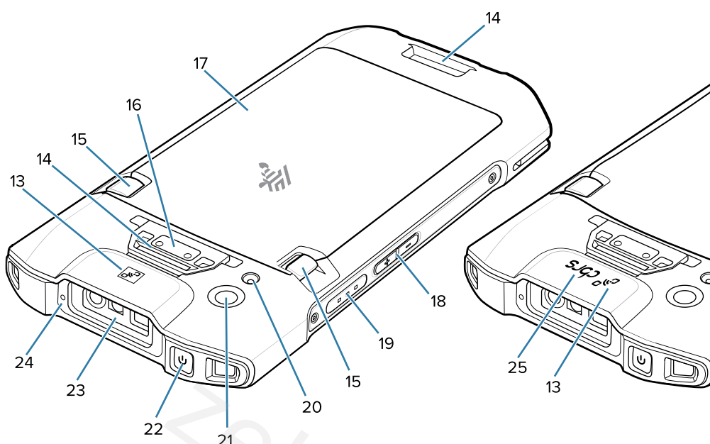
Figure 2 Rear View
