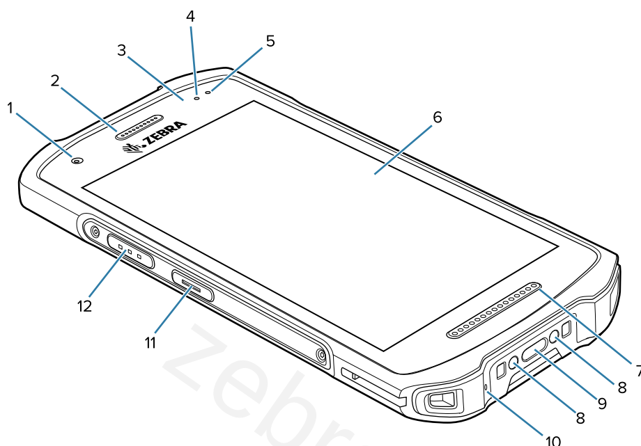
Figure 1 Front View
