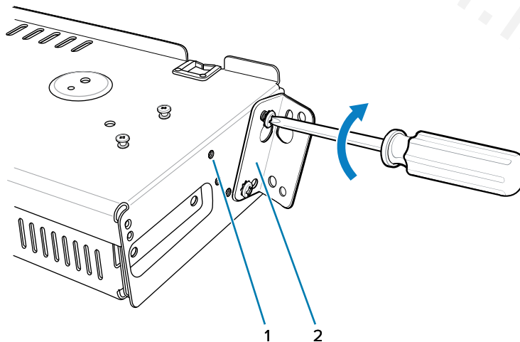
Figure 41 Flange 25° Position (4-Slot Battery Chargers)
