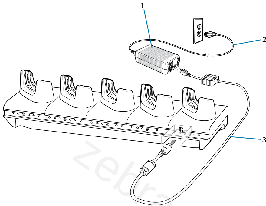
Figure 42 5-Slot Charge Only Cradle Setup
