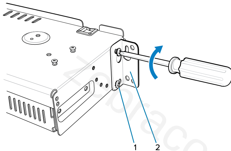
Figure 49 Flange Horizontal Position (5-Slot Cradles)
