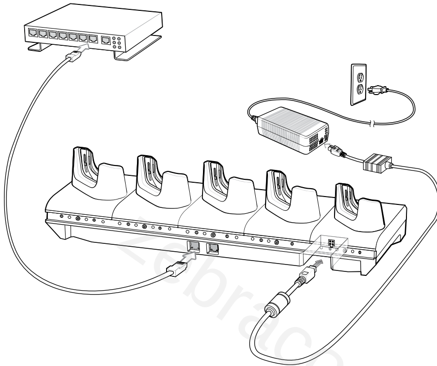
Figure 45 5-Slot Ethernet Cradle Setup
