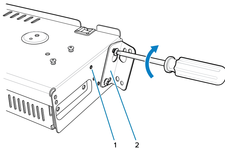
Figure 50 Flange 25° Position (4-Slot Battery Chargers)
