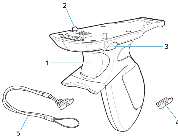
Figure 51 Trigger Handle
