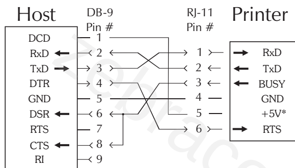
Female DB-9 to RJ-11
