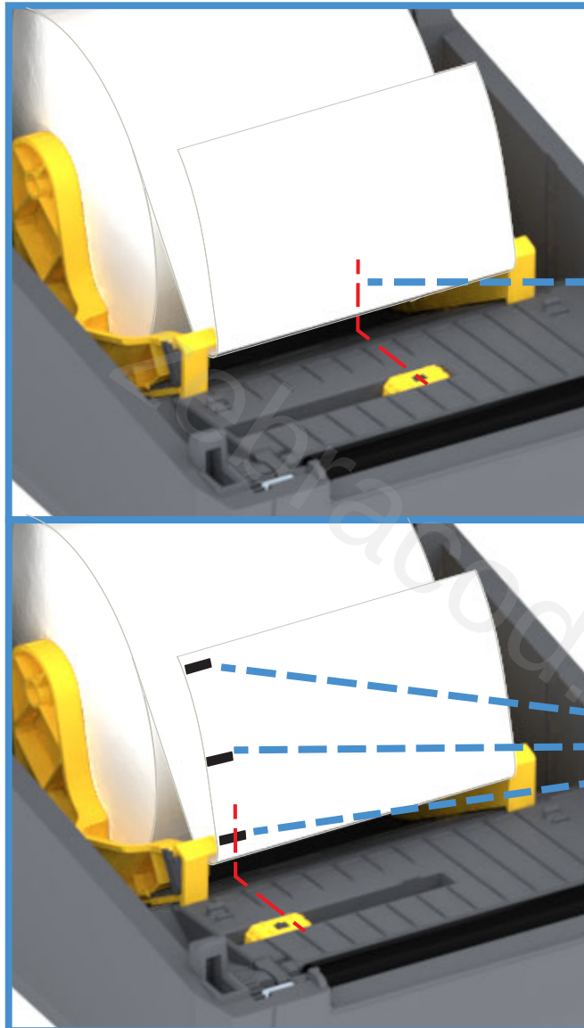
Default - Web (Gap) Sensing Standard Operating Position
