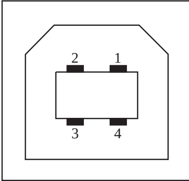
Figure 17 USB -B
