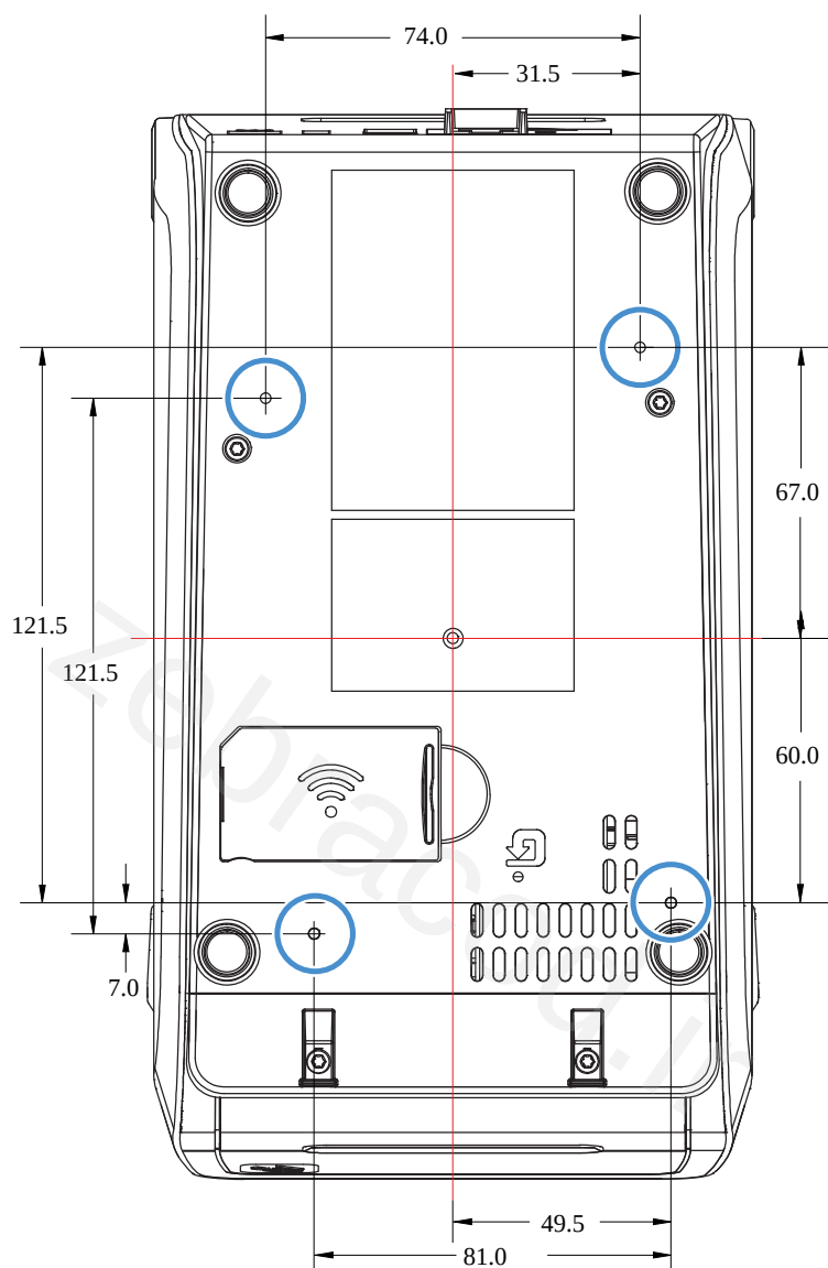
Figure 24 ZD411T Standard Mounting (dimensions in millimeters)
