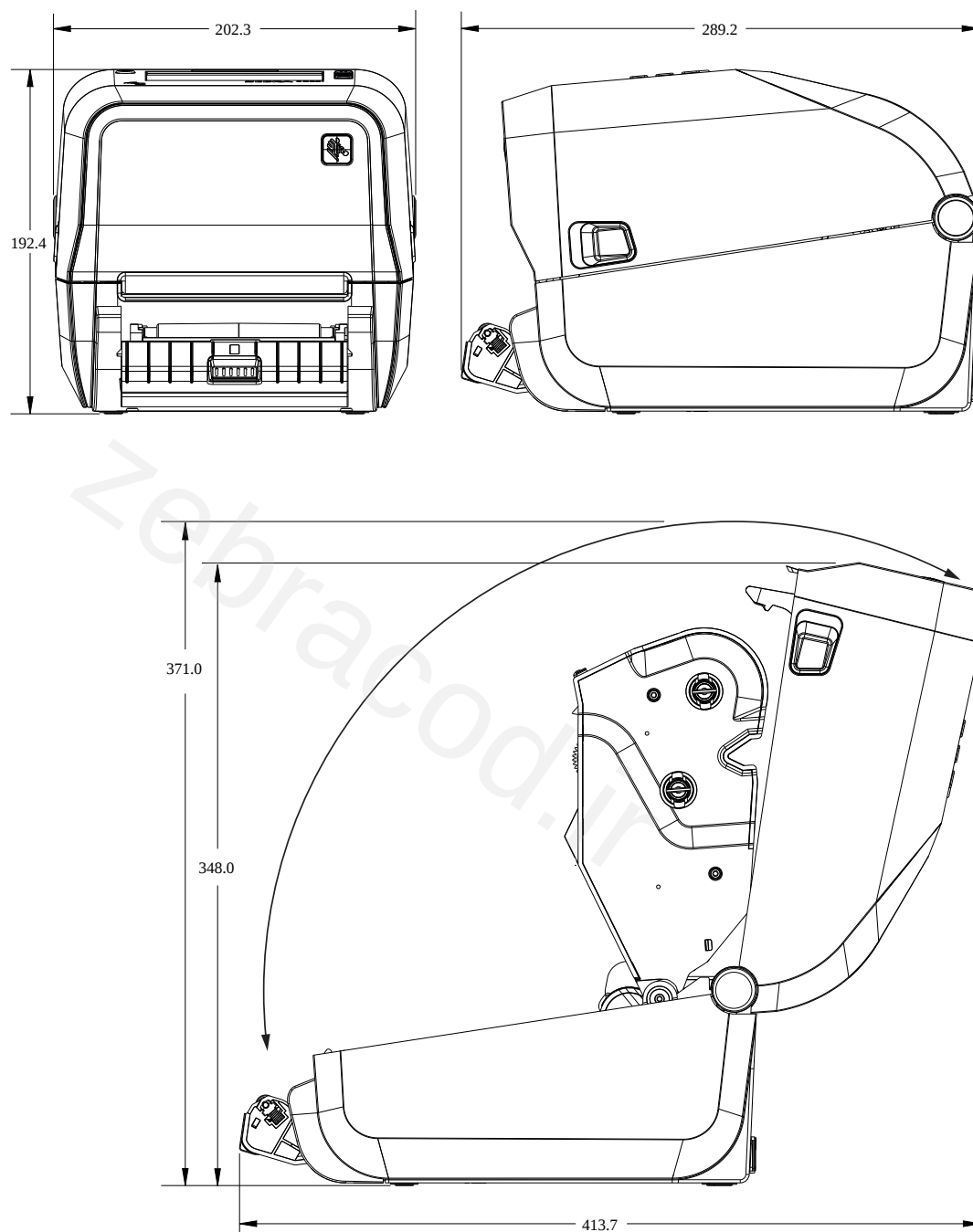
Figure 21 ZD621 / ZD421 Thermal Transfer Models – Dimensions for Printer with the Label Dispenser Option Installed
